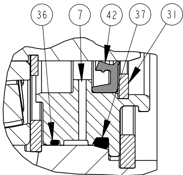
SINGLE SHAFT SEAL ASSEMBLY P2-145-0210-01□ SECTION A-A SCALE 1:1
